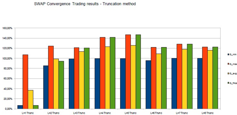
Figure 12. Comparison of minimum, maximum, average and final return on historical U.S. swap data of the truncation method for sparse, mean reverting portfolios of cardinality 1 to 8
