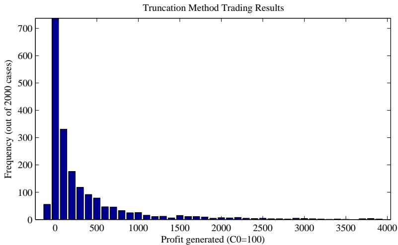
Figure 10. Histogram of profits achieved over 2000 different generated VAR(1) series. Note that in 30 cases the profit exceeded $4000 (not shown on the histogram) with maximum profit of $12.6 million reached
