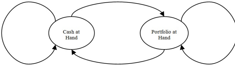
Figure 3. Trading as a walk in a binary state-space
