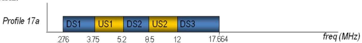
Figure 5 - Example band plans for profile 17a
