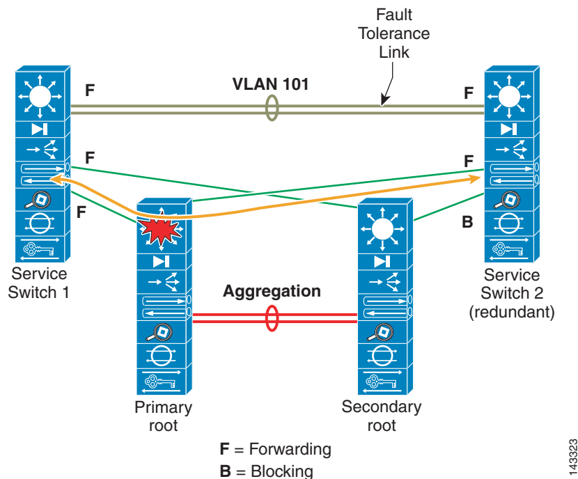
Figure 2-13 Redundancy with the Service Layer Switch Design
