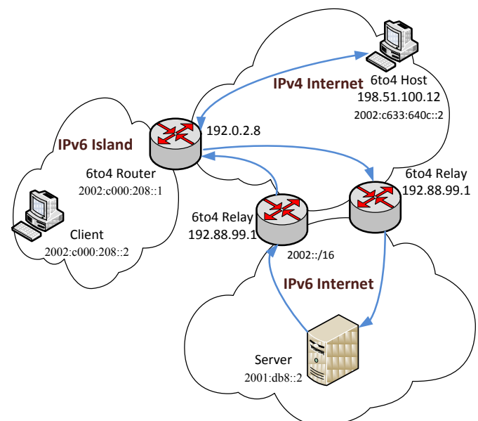
Fig. 1. Sample network for the demonstration of 6to4
