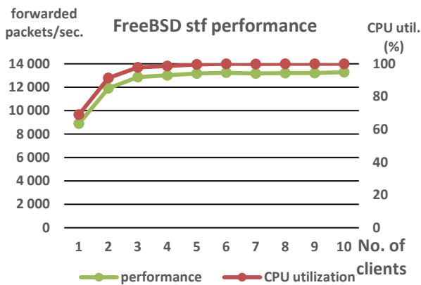
Fig. 14. FreeBSD stf performance and CPU utilization
