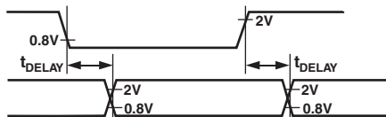
Figure 2. Voltage Reference Levels for Timing
