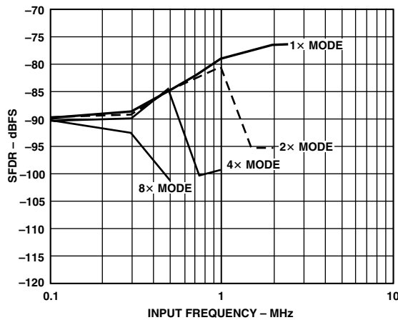
Figure 16. SFDR vs. Input Frequency ( f_{\text{CLOCK}} = 10 MSPS)
