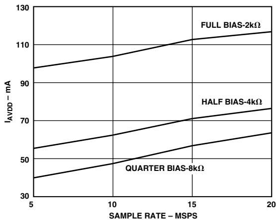
Figure 64. I_{AVDD} vs. Sample Rate ( AVDD = +5 V , Mode 1x-4x)
