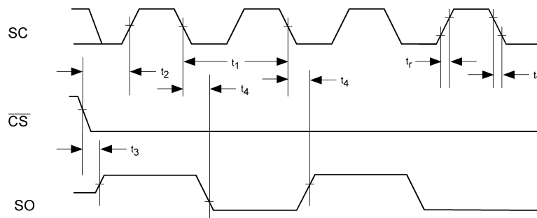
FIGURE 2. Data Output Timing Diagram
