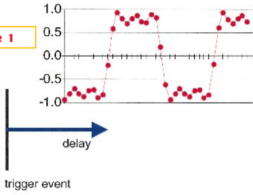
A variable monostable causes successive sample points to occur at an increasing distance from the trigger event.
