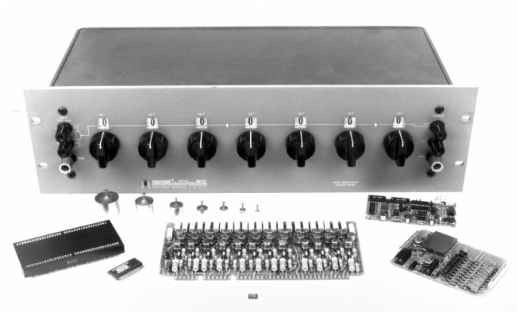
Historically significant D/A converters include: weight set (center left); more-than-23-bit Kelvin-Varley divider (large box); hybrid, board, and modular types; and the LTC1595 IC (fore-ground).
